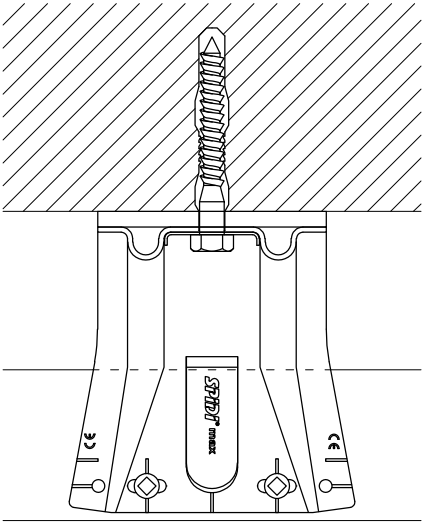
SLIDING POINT
