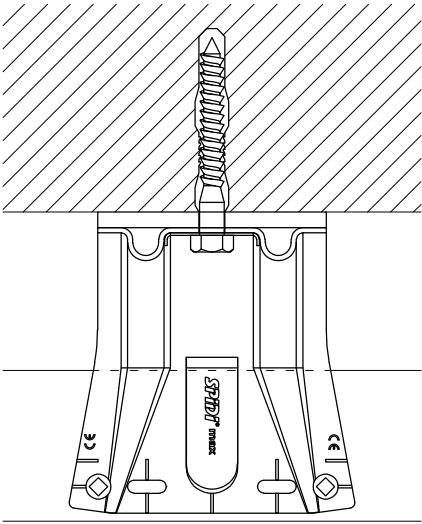
FIXED POINT
