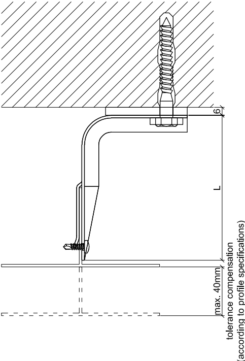
TOLERANCE COMPENSATION
