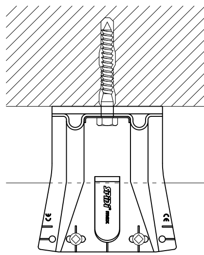
SLIDING POINT
