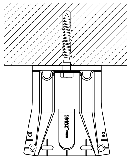
FIXED POINT
